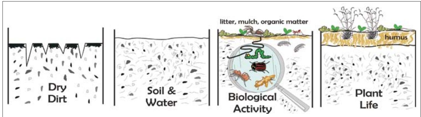
Figure 1. Restoring the soil’s “sponge” capacity restores the watershed.
